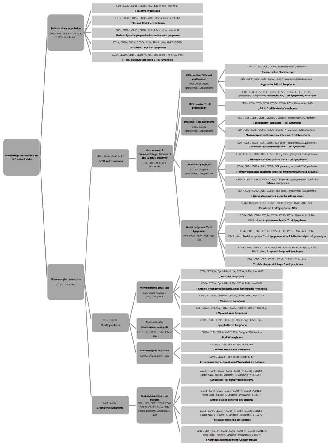
Supplementary Fig. S1. A schematic of lymphoid neoplasm subtyping using an immunohistochemistry profile.
