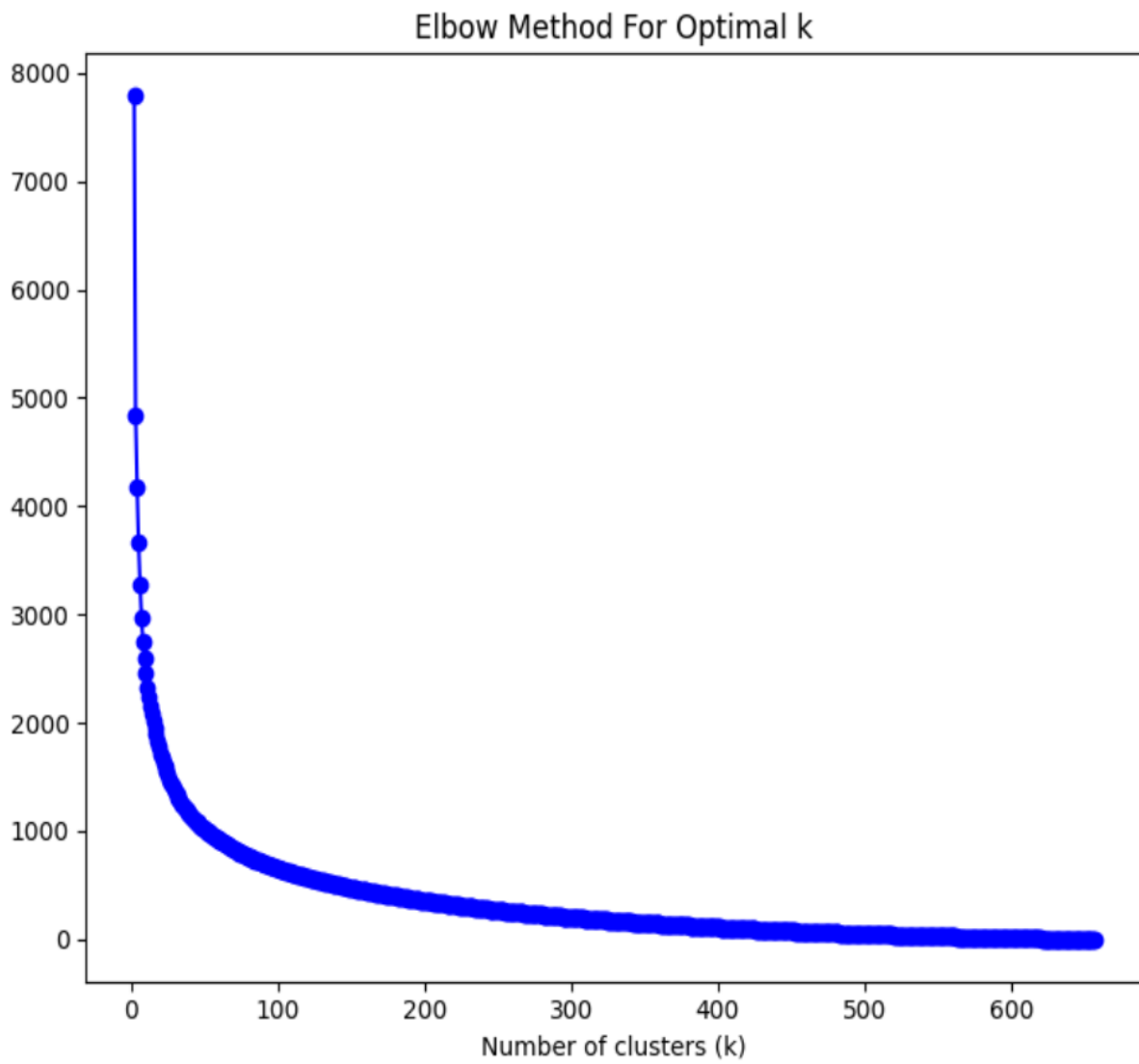
Supplementary Fig. S1. Elbow method for finding the optimal number of cluster for hierarchial clustering of common historic clusters across The Cancer Genome Atlas samples.
